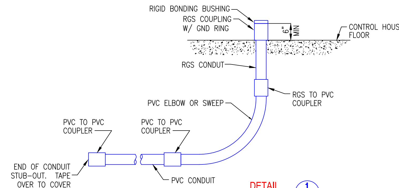
DETAIL 1 TYPICAL STUB-UP WITH ABOVE GRADE CONTROL CONDUIT IN CONTROL HOUSE
